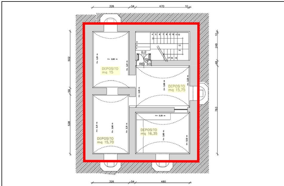
PIANO INTERRATO
