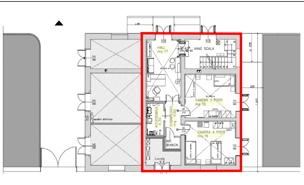
PIANO TERRA
